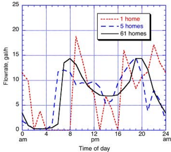
Figure 2. Hourly Flow Rates Measured Over a 24-hour Period.
